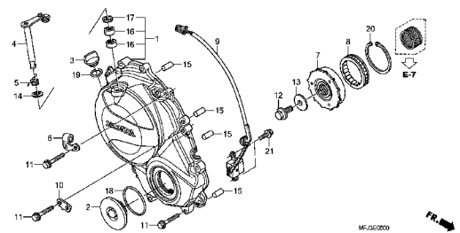
GENERATOR COVER
