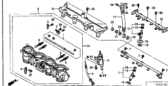
THROTTLE BODY (CBR600RR3/4)
