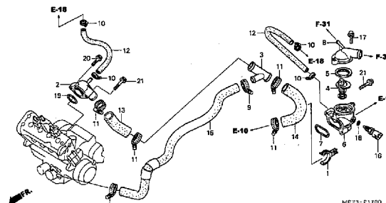
THERMOSTAT
