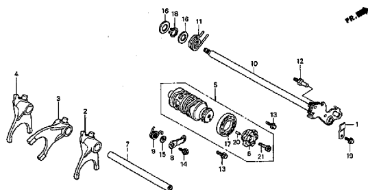
GEARSHIFT DRUM
